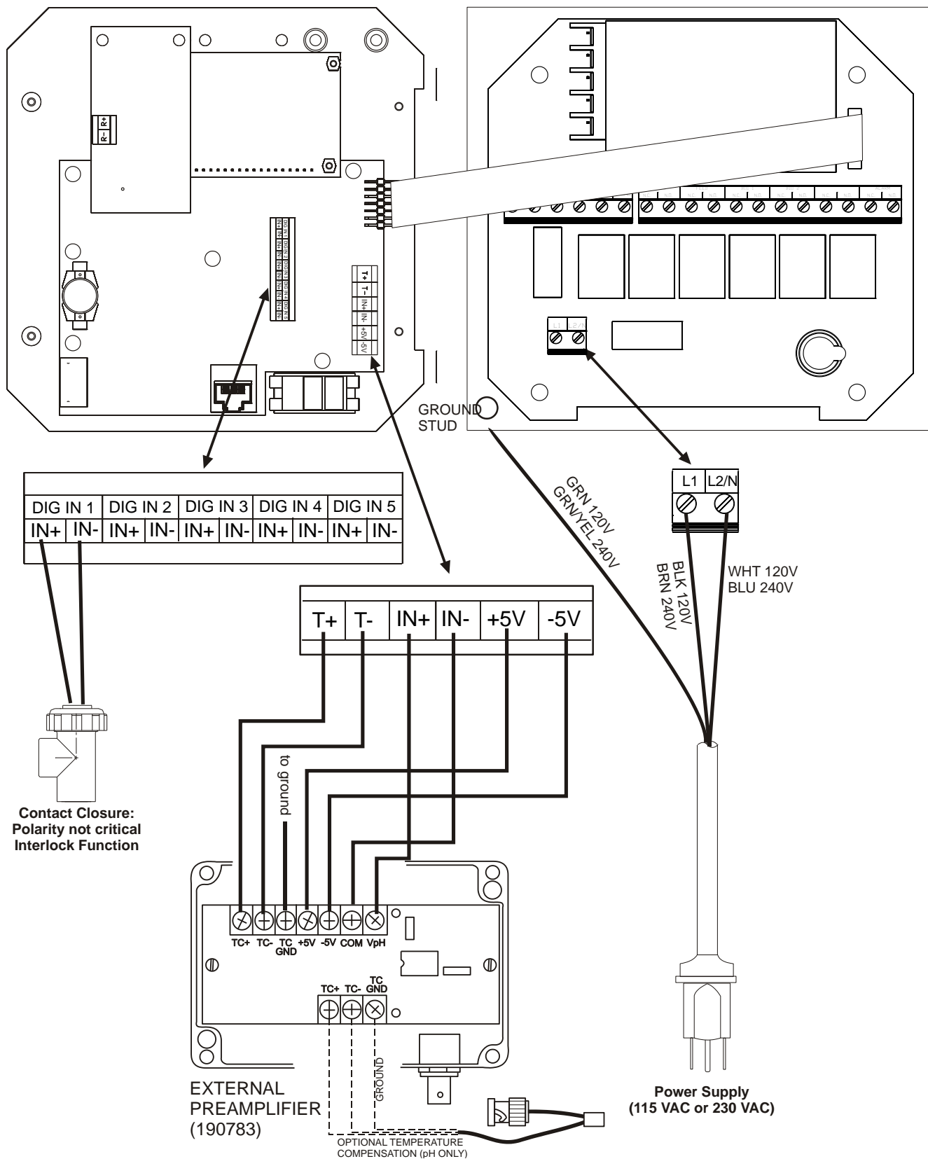
Figure 3b WPH Inputs using pH/ORP Electrode/External Preamplifiers
