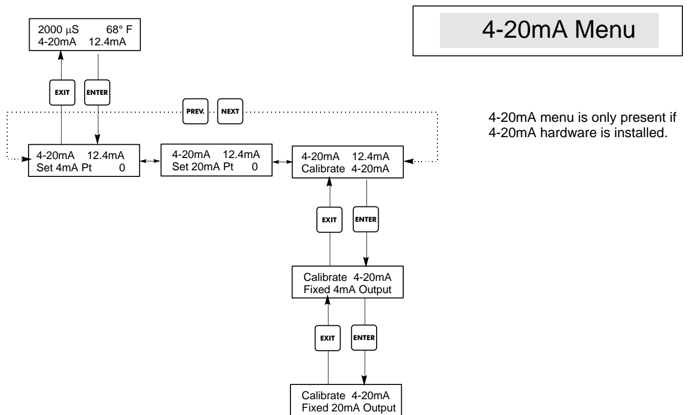
Figure 17 4-20 mA Menu
