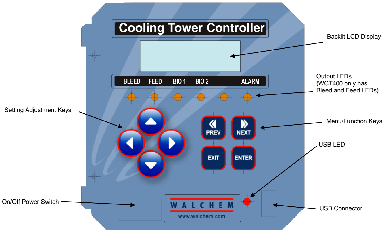
Figure 5 Front Panel
